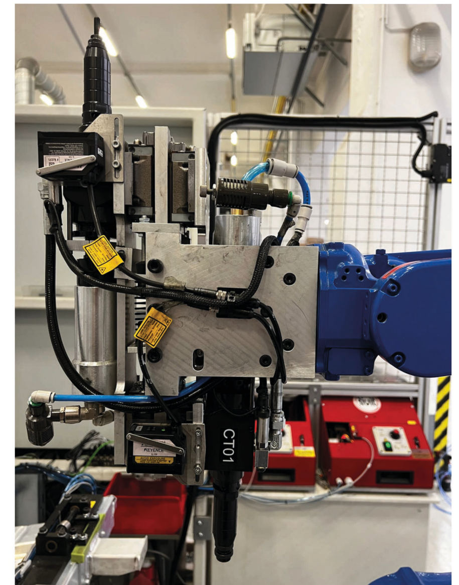
Robot riveting
