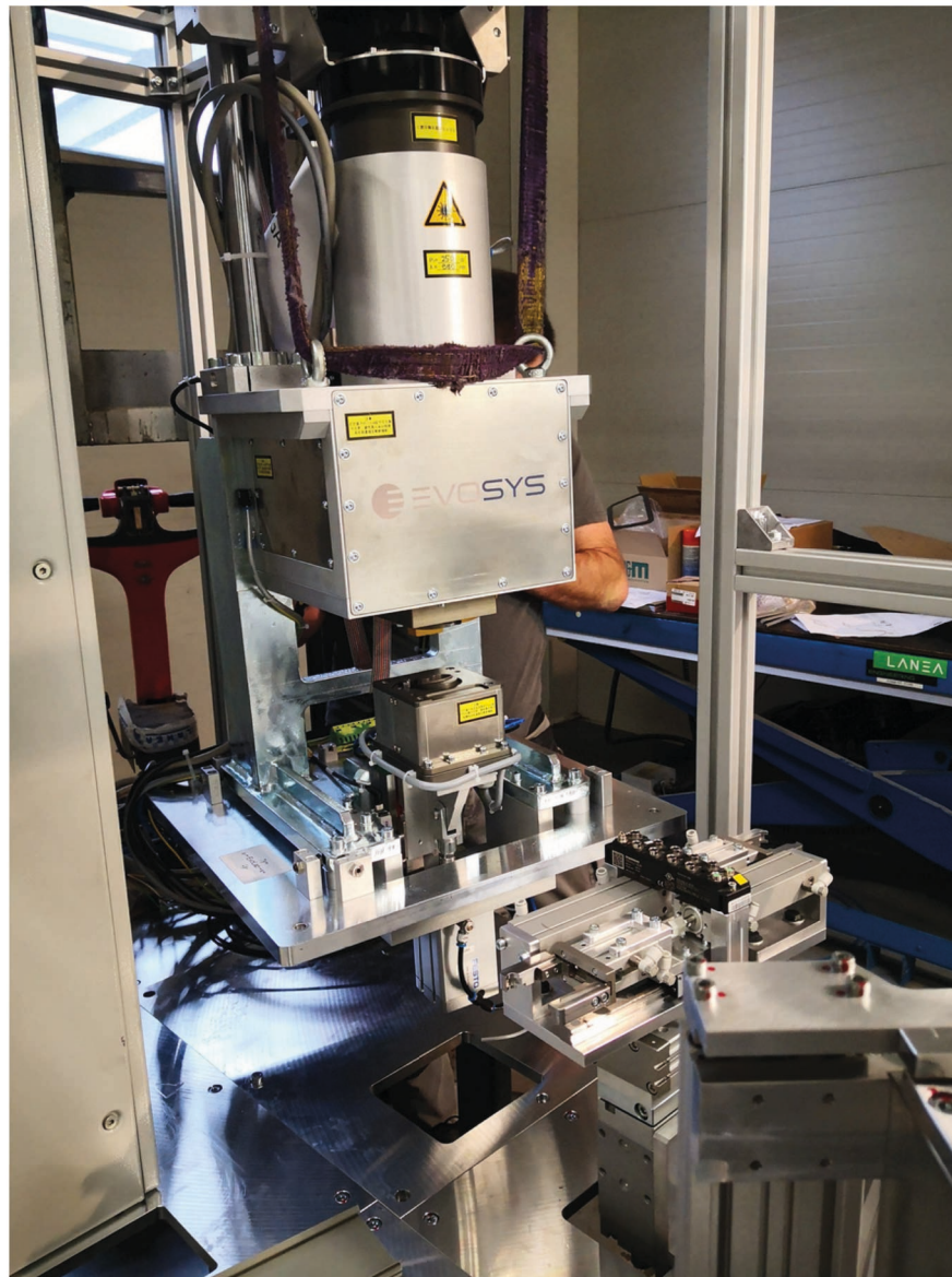
Laser welding plastic and metal parts
