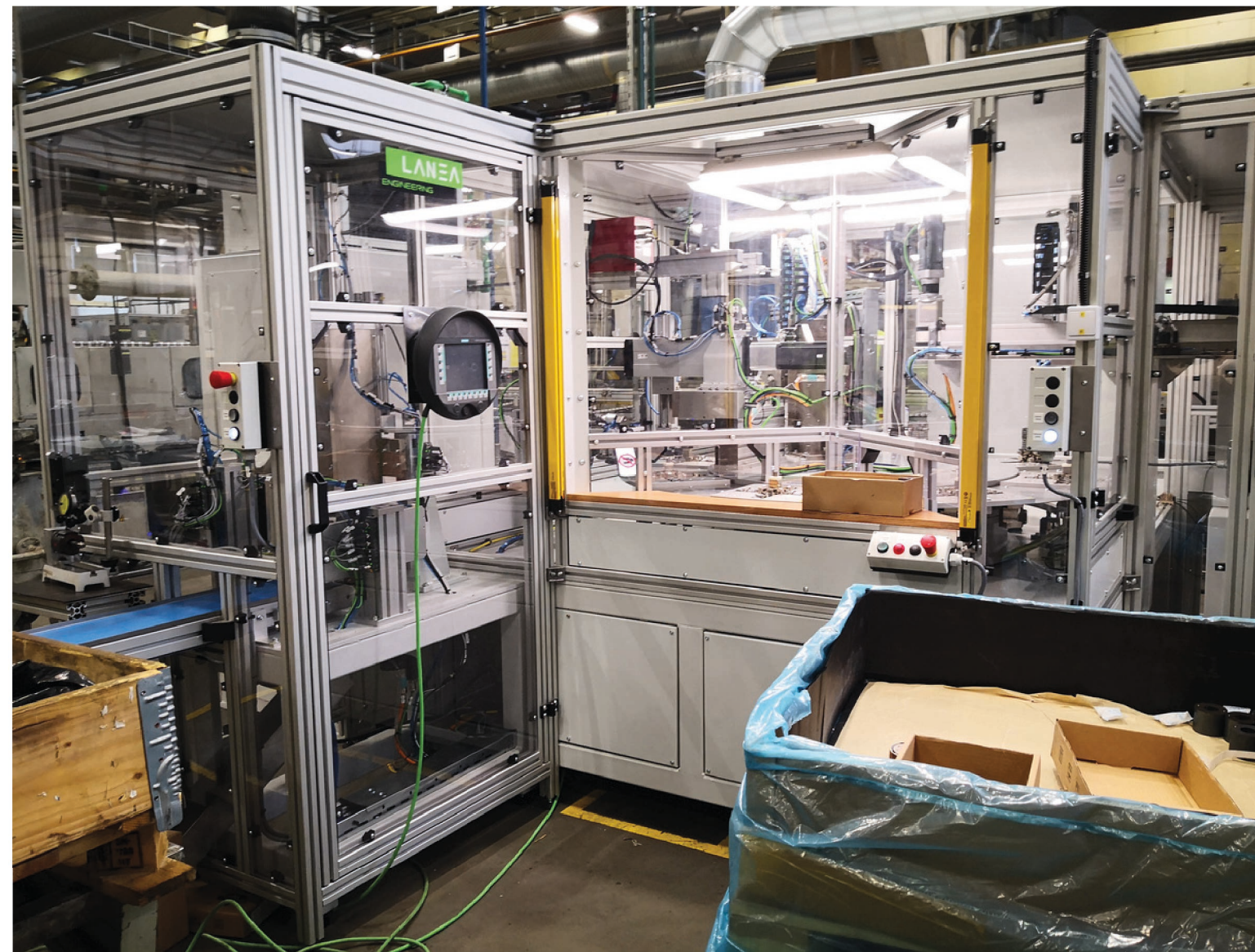
Rotor assembly line
