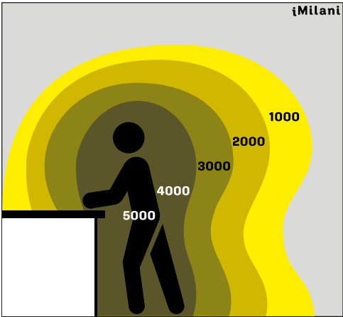
Electromagnetic field surrounding a person with an electrostatic charge (values in Volts)
